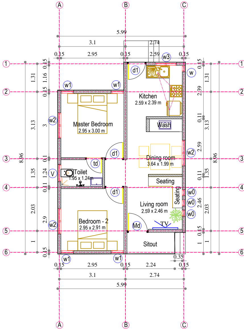
GROUND FLOOR PLAN FLOOR AREA : 49.09 SQM (528 sqft)
