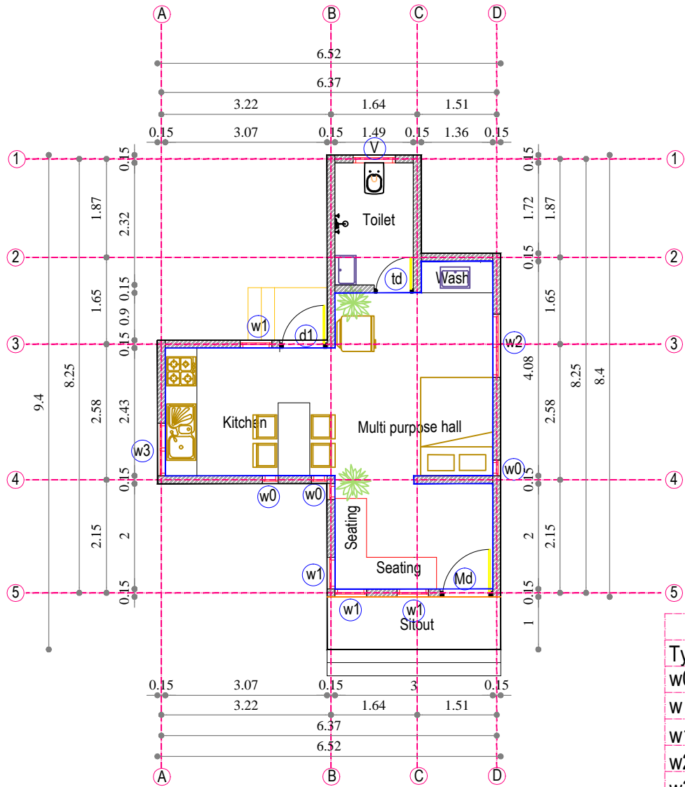
GROUND FLOOR PLAN AREA : 36.97 SQM (397.97 Sqft) CARPET AREA : 29.58 SQM
