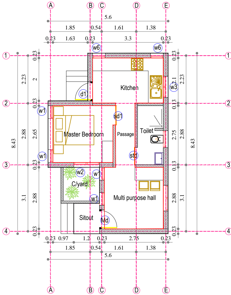
Single unit dwelling (1BHK) AREA : 37.45 SQM
