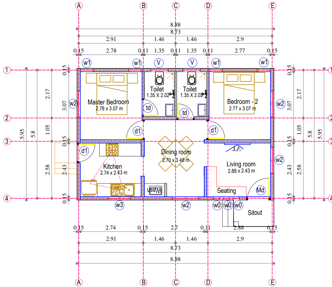
GROUND FLOOR PLAN FLOOR AREA : 48.90 SQM (526.16 sqft) CARPET AREA : 39.1 SQM
